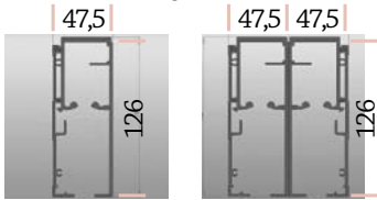
single track ceiling and wall
